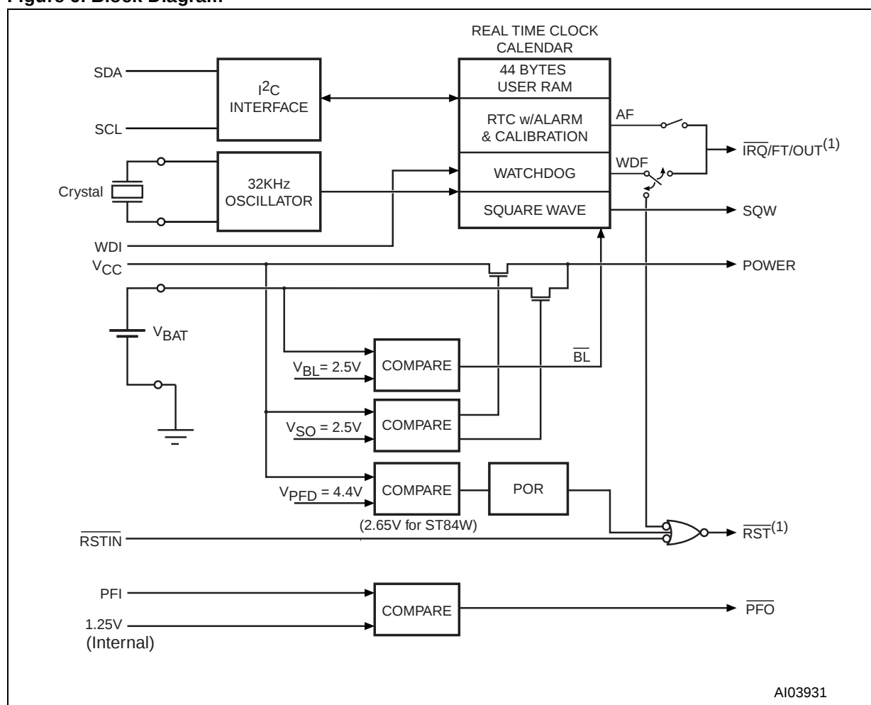
Figure 6. Block Diagram
